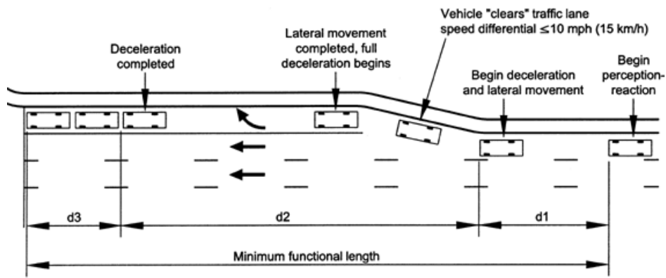
Figure 2-8: Functional area distance of an intersection approach (Rodegerdts et al. 2004).
